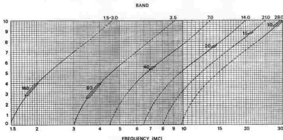
Figure 3-2. Preselector Tuning Ranges
