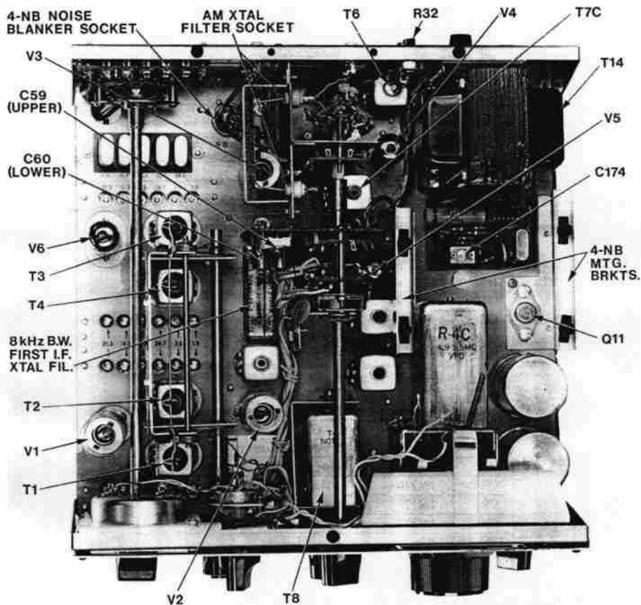
Figure 5-1. Alignment Locations, Top View
