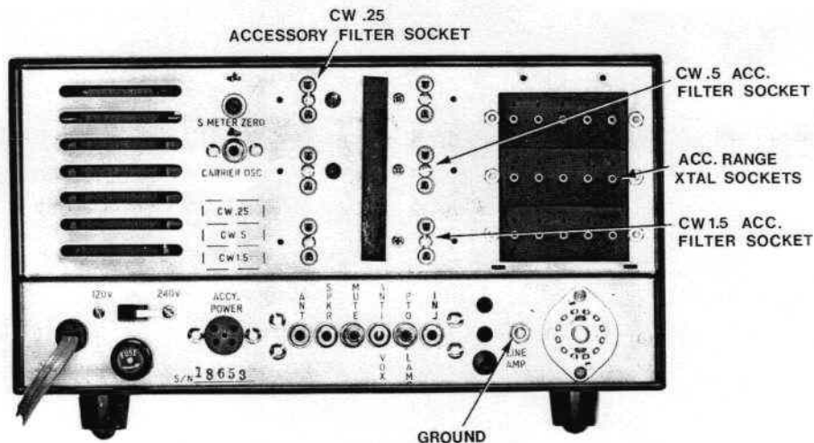
Figure 2-2. Rear Chassis Controls
