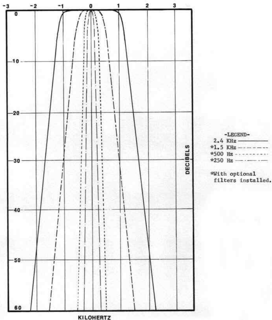
Figure 3-4. SSB and CW Selectivity Curves
