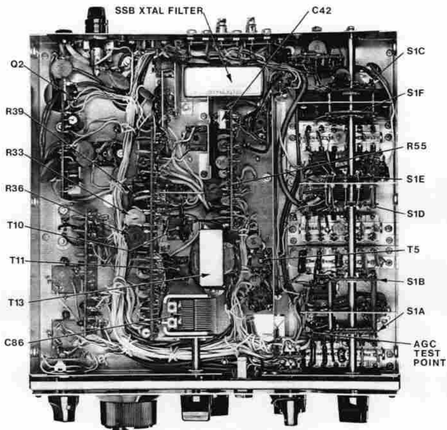
Figure 5-2. Alignment Locations, Bottom View
