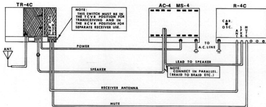
Figure 2-3. Connecting the TR-4C Transceiver
