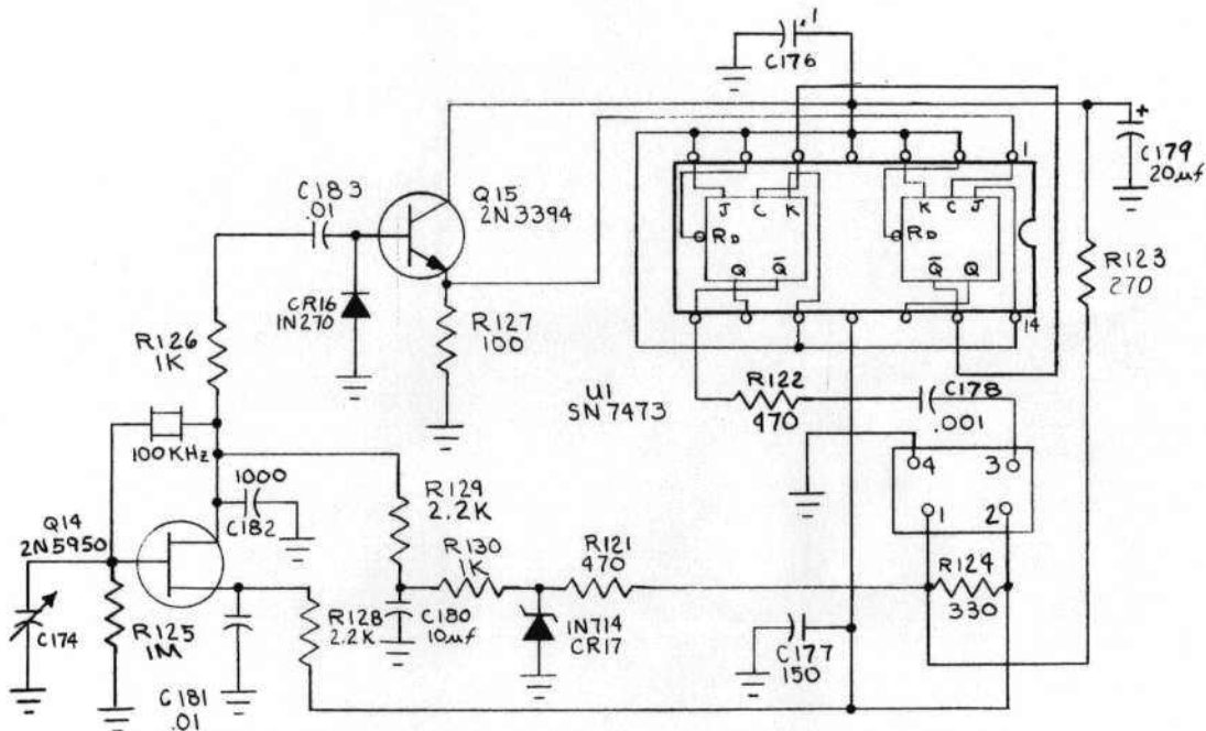
RCC4 CRYSTAL CALIBRATOR PART OF R-4C
