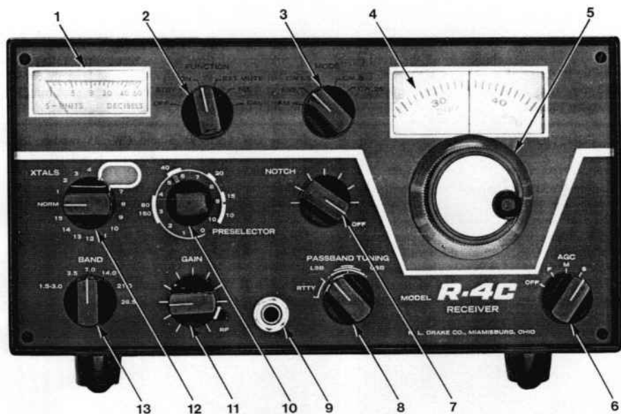
Figure 3-1. Front Panel Controls
