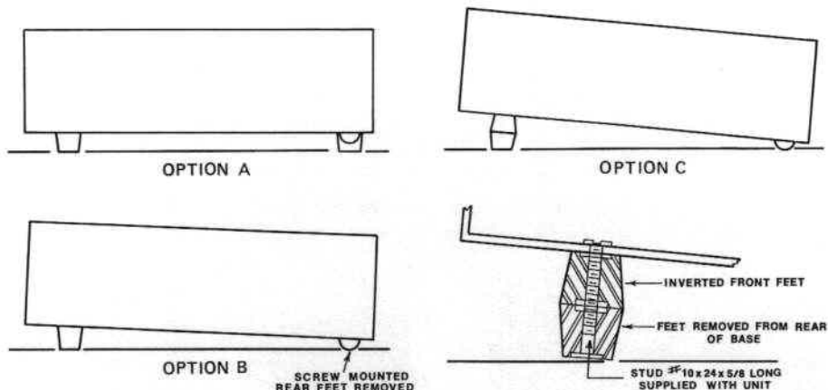
Figure 2-1. Viewing Angle Options
